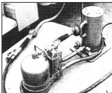
1. Air-Hydraulic Pump and 50-ton jack. Air supplied to the pump develops hydraulic pressure to lift the jack. This equipment is essential in servicing extra-heavy construction equipment.
